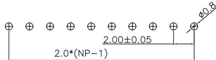
PCB LAYOUT
