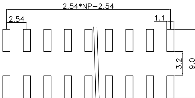
PCB LAYOUT
