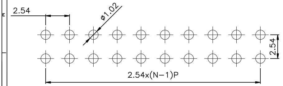
PCB LAYOUT
