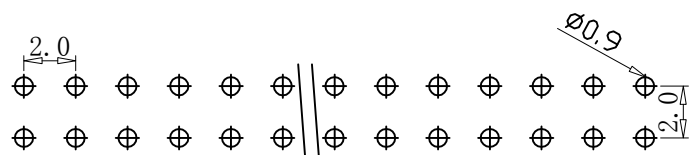
PCB LAYOUT
